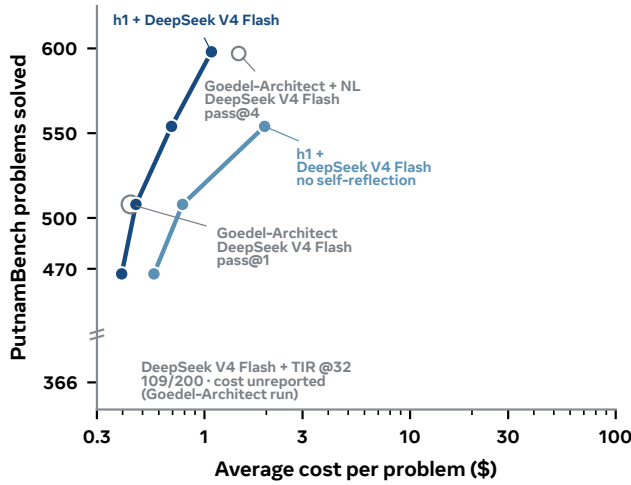
Figure 7 Reflection substantially improves h1’s coverage, exceeding Goedel-Architect’s pass@4 coverage at lower estimated cost. With the same DeepSeek V4 Flash model, h1 also substantially outperforms Goedel-Architect’s tool-integrated reasoning (TIR) baseline, showing that its baseline understates what a simple agent can achieve.
