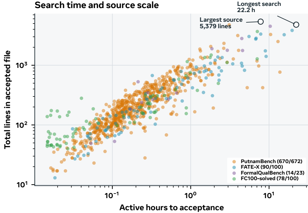
Figure 32 Search time and total file length across 852 accepted proofs. GPT-5.5 on PutnamBench; GPT-5.6 Sol on FATE-X, FormalQualBench, and FC100-solved.
