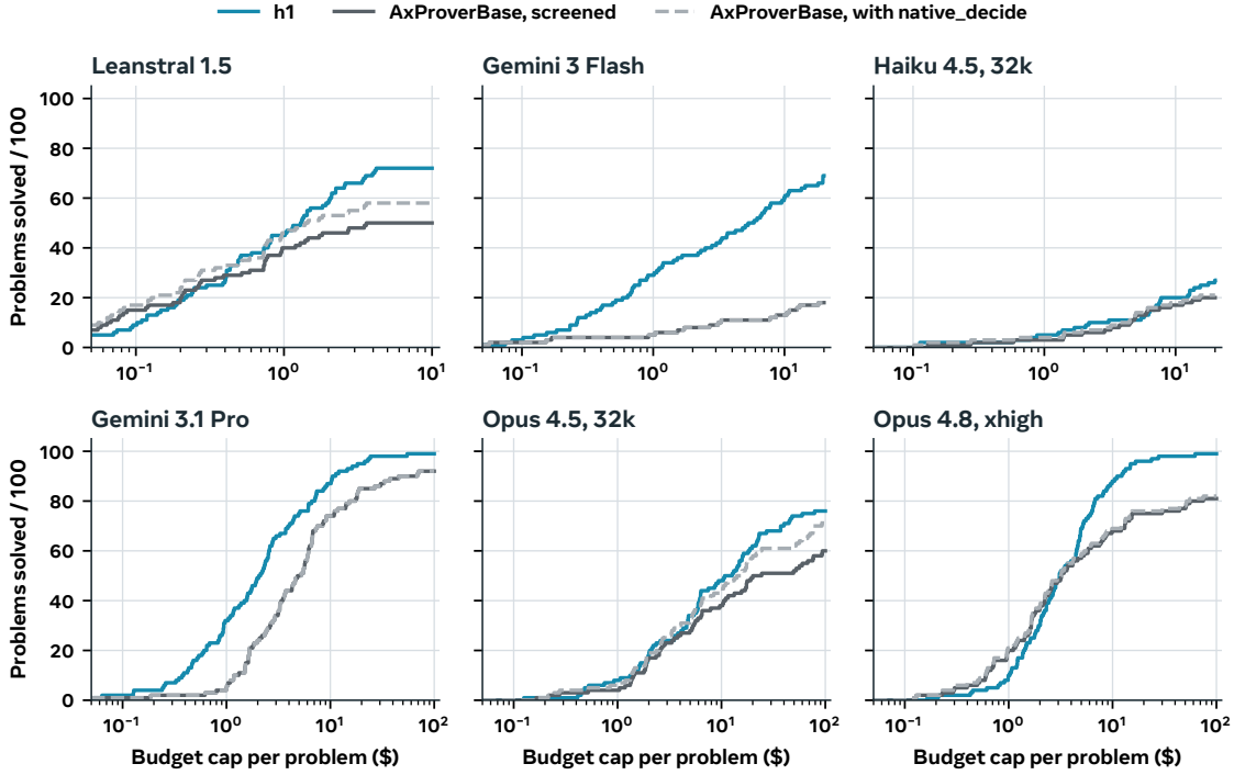
Figure 17 h1 overtakes AxProverBase as the budget grows across the six settings in Figure 5. AxProverBase is shown both before and after screening out proofs using native_decide ; overlapping lines indicate no screened solves. All h1 solves pass external validation.
