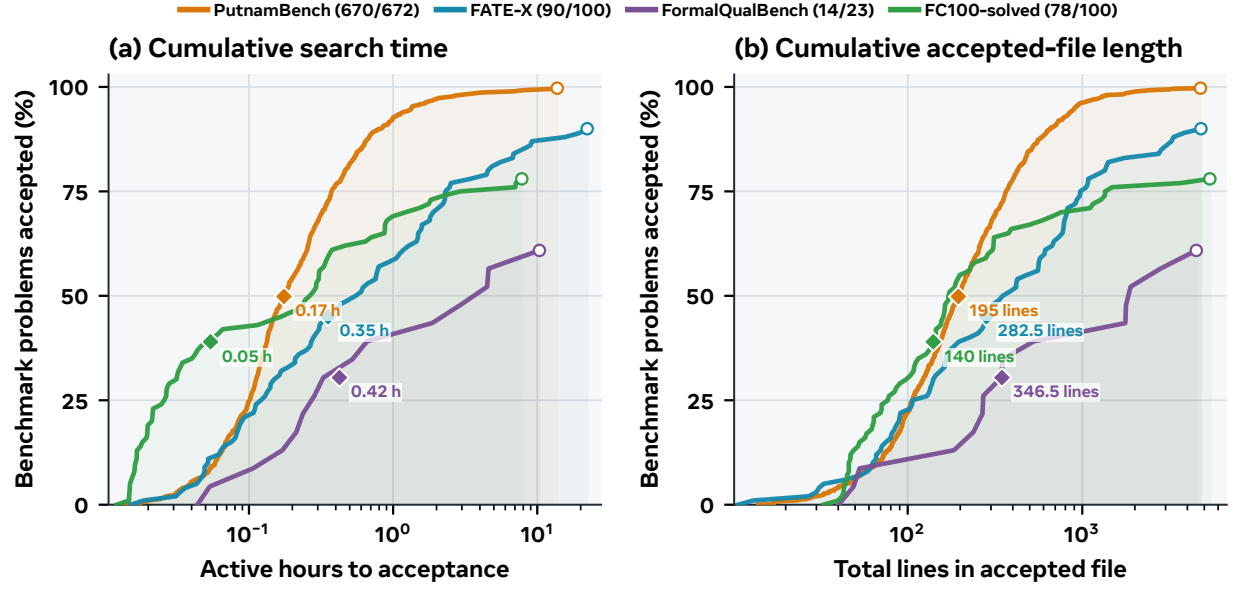
Figure 31 Cumulative distributions of time to acceptance and accepted-file length. The runs are those in Figure 30. Counts are divided by all attempted problems, so each curve ends at the run’s acceptance percentage. Diamonds mark medians among accepted proofs.
