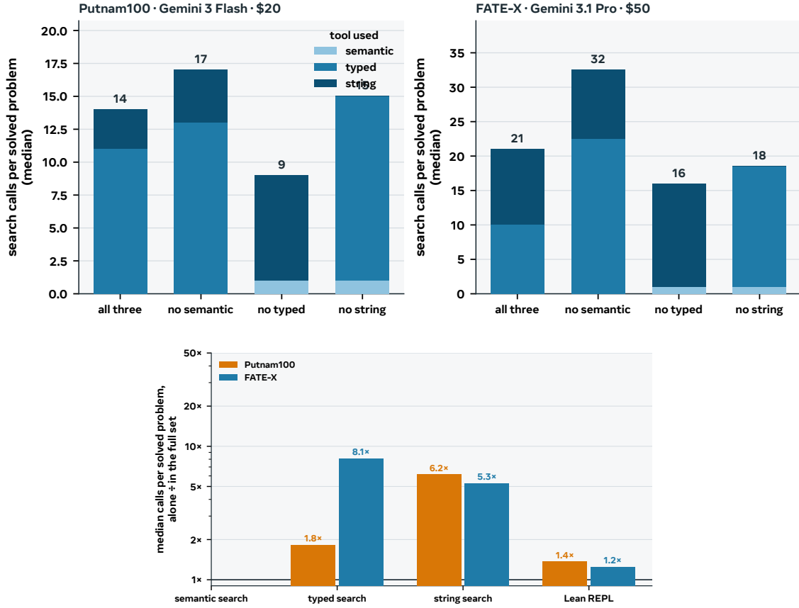
Figure 26 Tool use when search and execution capabilities change. Top: median calls to each search tool among problems solved by each configuration; stacked heights sum these tool-specific medians. Bottom: each tool’s median call count when it is the only additional capability, divided by its median with all tools available. These comparisons use each configuration’s own solved problems.
