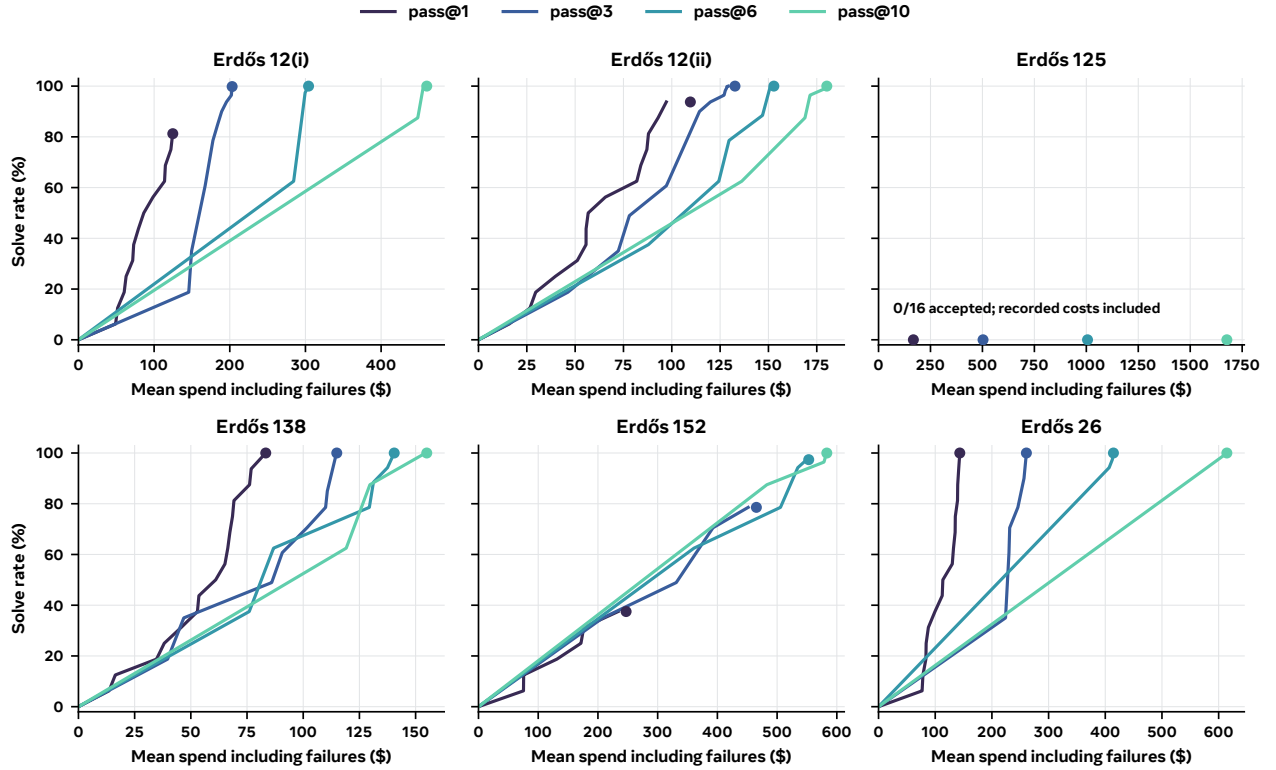
Figure 14 The trade-off between longer attempts and repetition varies by problem. The same unconditional-cost calculation as Figure 13, shown separately for each of the six Erdős problems. Lines join nondominated observed points; circles mark terminal results. All groups contribute to cost, including those that terminate in errors. Horizontal scales differ across panels. On Erdős 152, pass@10 reaches 87.5% at $483 and leads the tested smaller values of k until pass@6 reaches 94.2% at $535.
