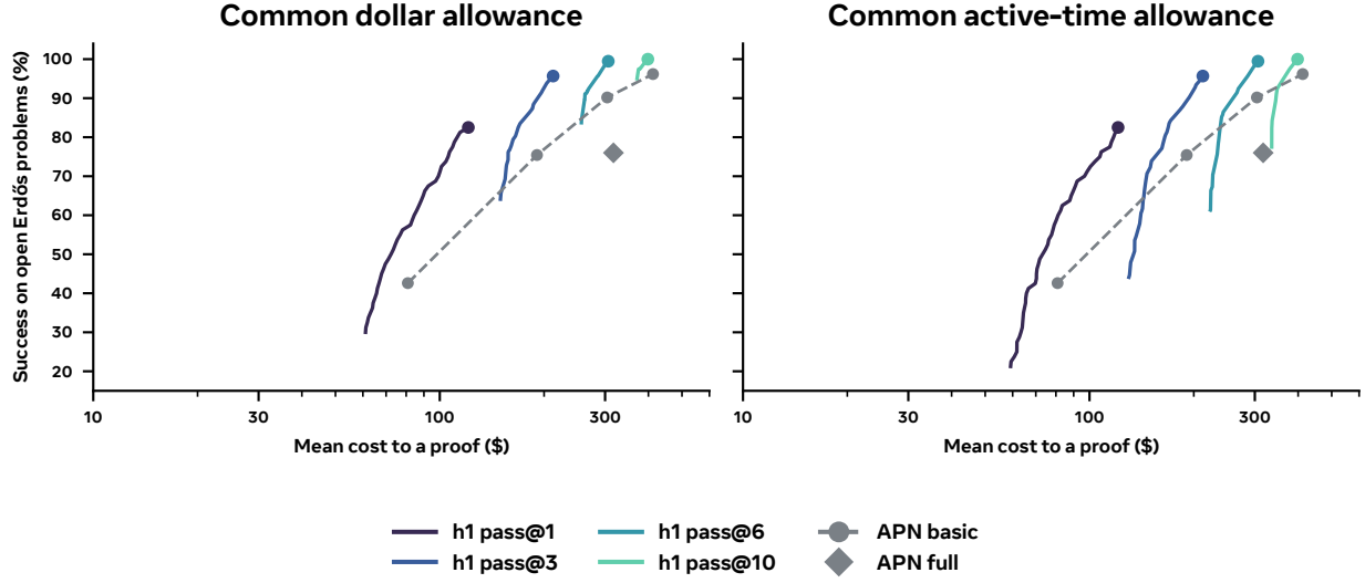
Figure 15 Dollar and time alignment give the same terminal comparisons. Both panels average the same five problems equally and count each group’s cost up to its first eligible proof. Only the common allowance across problems changes. Solid curves vary that allowance at fixed k ; circles mark terminal results. APN’s published points are identical in both panels.
