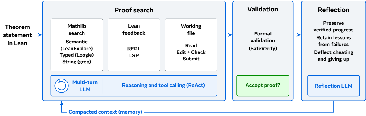
Figure 2 h1: a simple harness that scales. An LLM agent edits a Lean file through reasoning and tool calls (ReAct; Yao et al., 2023) until it submits or reaches the T -turn limit, forcing submission. An external validator then checks the proof. On failure, a reflection LLM compacts the transcript and feedback for the next iteration. The loop provides Lean tools without prescribing a proof search structure. Search uses LeanExplore (Asher, 2025), Loogle (Breitner, 2023), and grep; proof fragments run in the Lean read-eval-print loop (REPL) (leanprover-community, 2023); the language server (LSP) reports goals and definitions; SafeVerify (GasStationManager, 2024) performs validation.
