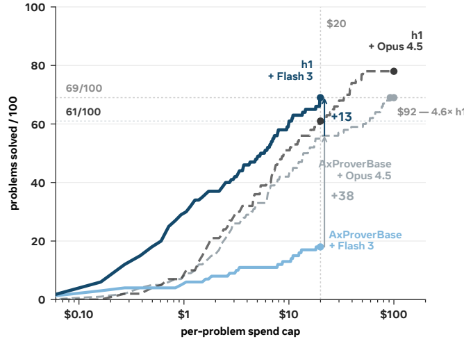
Figure 19 PutnamBench subset solve rates for h1 and AxProverBase as the budget increases. h1 with Opus 4.5 solves 61 problems at the $20 per-problem cap.
