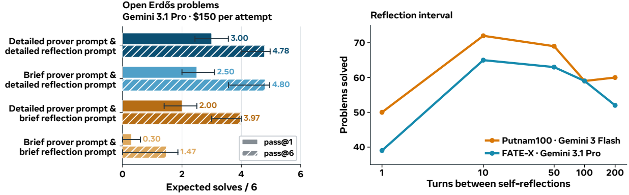
Figure 4 (Left) Detailed prompts sustain progress on open problems. With Gemini 3.1 Pro on six open Erdős problems and a $150 cap per attempt, a single attempt with detailed prover and reflection prompts, which among other things deflect giving up and cheating, outperforms six attempts with brief ones. (Right) Moderate numbers of turns between reflections outperform both extremes. Solves with Gemini 3 Flash on Putnam100 ($20 cap) and Gemini 3.1 Pro on FATE-X ($50 cap) as the number of turns between reflections varies.
