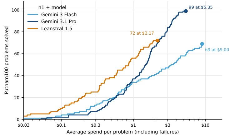
Figure 16 The most economical model depends on the target solve rate. On the PutnamBench subset, Leanstral 1.5 supplies the frontier through 72 solves and Gemini 3.1 Pro extends it to 99, while Gemini 3 Flash lies below their combined frontier. Each curve varies the per-problem cap; cost averages all 100 problems, including failures. Dots mark full-run endpoints. Leanstral costs are API-equivalent estimates using a measured 65% average cache rate at maximum context length.
