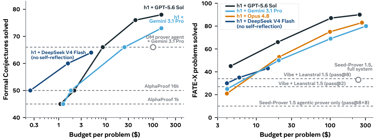
Figure 8 Figure 3 with the DeepSeek V4 Flash setting labelled. FC100-solved (left) and FATE-X (right); the DeepSeek V4 Flash runs use h1 without self-reflection.
