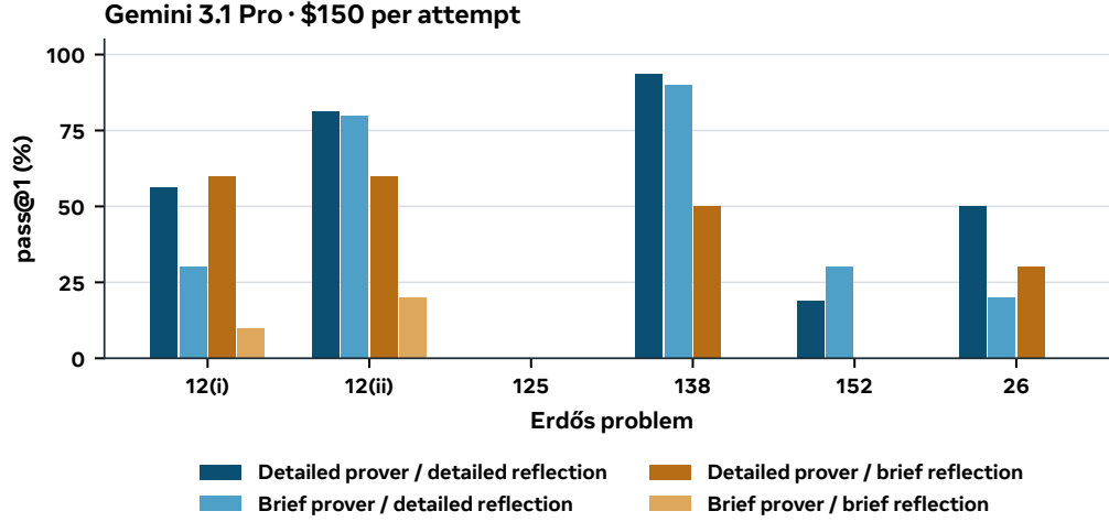
Figure 10 Per-problem success under different prompts for the two LLM roles. The same runs and $150 cap as Figure 4; bars show pass@1, with all replicas in the denominator.
