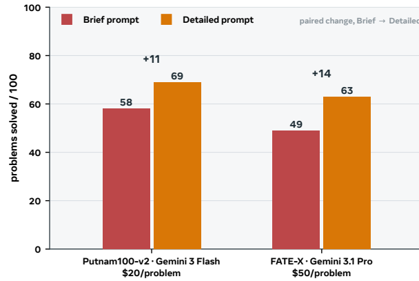
Figure 23 The detailed prompt improves solve rates on both ablation settings. Gemini 3 Flash on the PutnamBench subset ($20 per problem) and Gemini 3.1 Pro on FATE-X ($50); all 100 problems per arm remain in the denominator, including crashes. The prompt variants are specified in Appendix B.2.
