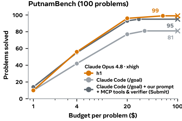
Figure 6 Claude Code improves with our Lean tools but still falls short of h1 on the PutnamBench subset. With Opus 4.8, native Claude Code solves 81 problems; our prompt and Lean tools through MCP, in place of its built-in shell and file tools, raise this to 95, while h1 reaches 99. The FATE-X comparison appears in Figure 5, right.
