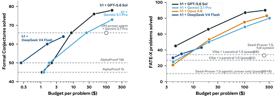
Figure 3 Generalist models reach frontier results through simple scaling. On FC100-solved (left) and FATE-X (right), increasing h1 ’s inference budget takes generalist models beyond published benchmark scores. On FC100-solved, h1 with Gemini 3.1 Pro matches the DeepMind (DM) prover agent’s score at a quarter of its budget cap; with GPT-5.6 Sol, it solves 78, and 90 on FATE-X. With DeepSeek V4 Flash, h1 surpasses AlphaProof on FC100-solved and Leanstral 1.5 on FATE-X. Baseline markers show the best published results as of August 27, 2026.
