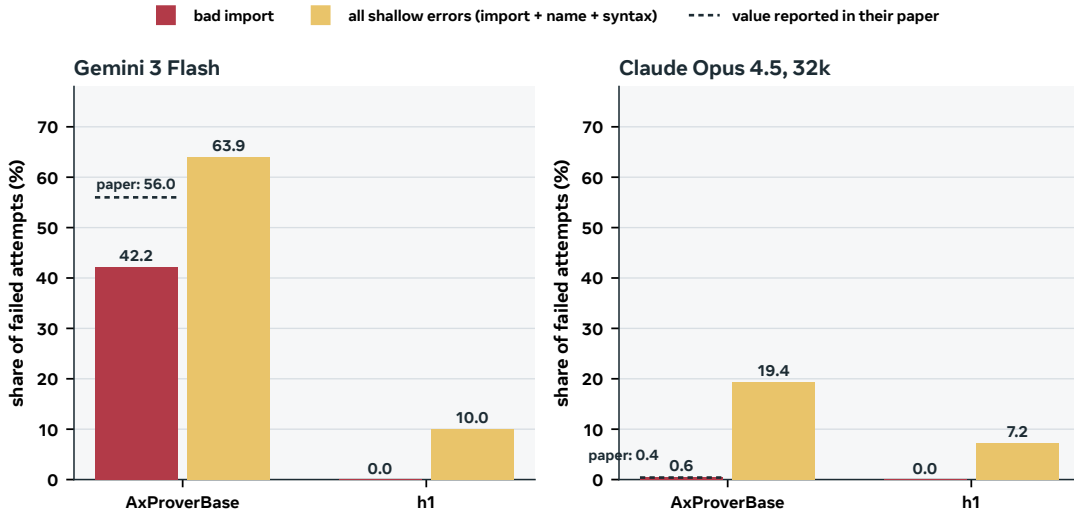
Figure 20 Bad imports consume proof-checking attempts. The fraction of failed builds whose first Lean error is a bad import is 42.2% for AxProverBase with Gemini 3 Flash and 0.6% with Opus 4.5; dashed lines show the paper’s reported 56% and 0.4%. h1 seeds the working file with import Mathlib and records no such failures.
