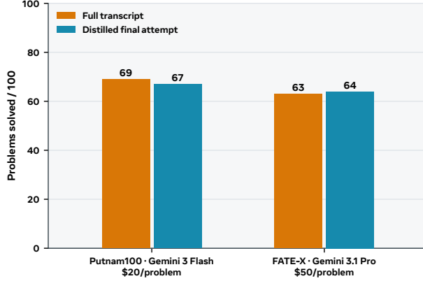
Figure 24 The two reflection LLM inputs yield similar solve counts in these runs. Full transcript versus distilled final attempt: 69 versus 67 solves on the PutnamBench subset with Gemini 3 Flash, and 63 versus 64 on FATE-X with Gemini 3.1 Pro. The per-problem caps are $20 and $50, respectively, including prover and reflection LLM calls; each arm contains 100 problems and one run.
