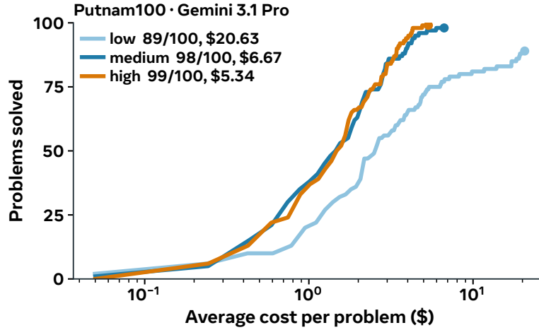
Figure 28 More reasoning per turn can make test-time scaling more efficient. Gemini 3.1 Pro on the PutnamBench subset with low, medium, and high reasoning effort. Curves plot solves against mean cost, including failed attempts; legends report final solve counts and mean costs.
