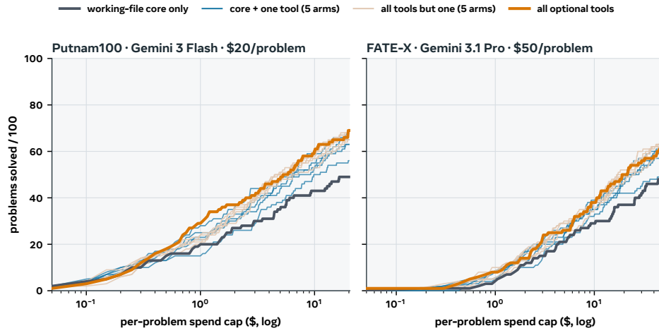
Figure 25 Solve rates under different tool configurations and inference budgets. Gemini 3 Flash on the PutnamBench subset ($20 per problem; left) and Gemini 3.1 Pro on FATE-X ($50; right). The working-file baseline permits editing and checking the proof file. Blue curves add one of five capabilities: semantic, type, or text search, the Lean REPL, or the language server. Pale curves remove one capability from the complete tool set. The working-file baseline generally solves fewer problems; the other configurations substantially overlap. On the PutnamBench subset, all tools retain all 49 working-file-baseline solves and add 20; on FATE-X, they retain 48 of 49 and add 15.
