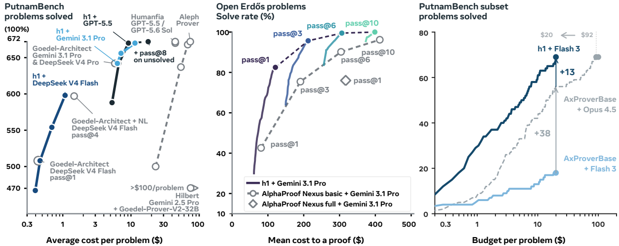
Figure 1 (Left) Simple scaling Pareto-dominates specialized systems. On PutnamBench (672 competition problems), h1 with DeepSeek V4 Flash Pareto-dominates Goedel-Architect’s best of four runs (pass@4) seeded with natural-language proofs. With GPT-5.5, it solves every solvable problem, as Humanfia and Aleph Prover do, at lower cost. (Middle) Longer attempts can outperform repetition. On five open Erdős problems, a single h1 attempt (pass@1) beats three attempts of AlphaProof Nexus’s basic agent (APN basic, pass@3) at lower mean cost per success, can be cheaper than repeating h1 itself, and Pareto-dominates the full APN system. (Right) Simple harness design is important for scaling efficiency and effectiveness. On a 100-problem PutnamBench subset, Gemini 3 Flash trails Opus 4.5 in the AxProverBase loop but overtakes it in h1 at matched budget through more efficient tool use and caching.
