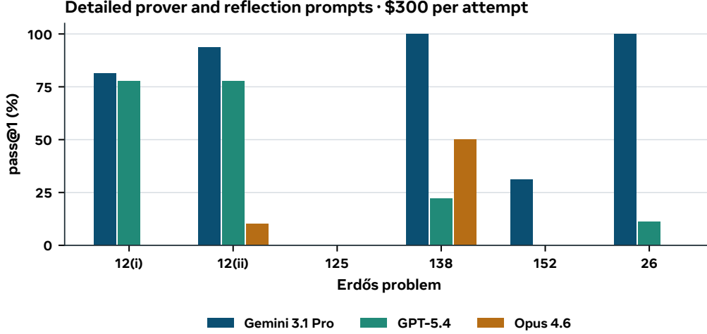
Figure 12 Per-problem success for the model comparison. Bars show pass@1 in the runs of Figure 11, with detailed instructions for both LLM roles and a $300 per-attempt cap.
