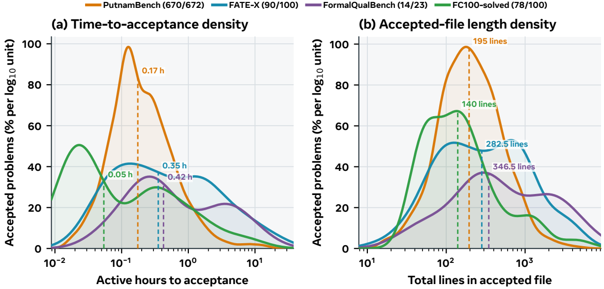
Figure 30 Time to acceptance and accepted-file length. The selected runs contain 670/672 accepted PutnamBench problems with GPT-5.5, and 90/100 on FATE-X, 14/23 on FormalQualBench, and 78/100 on FC100-solved with GPT-5.6 Sol: 852 accepted proofs in 895 attempts. Left: active hours to first acceptance. Right: total lines in the accepted Lean file. Densities are estimated in log 10 space and normalized so their area in that space equals the benchmark’s acceptance percentage. Dashed lines mark medians among accepted proofs.
