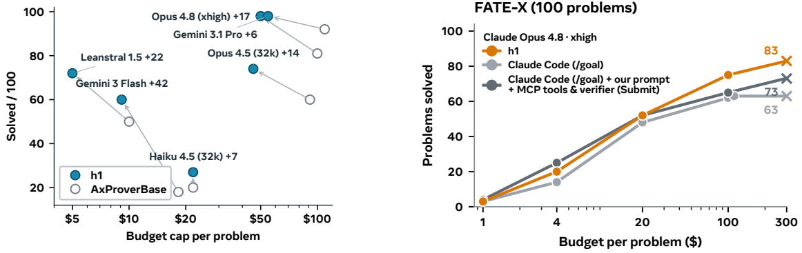
Figure 5 (Left) h1 Pareto-dominates AxProverBase on Putnam100. For each of six model settings, the arrow goes from AxProverBase to h1, labelled with the gain in solves at a comparable or lower budget cap. (Right) Claude Code improves with our Lean tools but still falls short of h1 on FATE-X. With Opus 4.8, replacing Claude Code’s built-in shell and file tools with our prompt and Lean tools through the Model Context Protocol (MCP) raises its solves from 63 to 73, while h1, which also enforces validation, repair, and reflection, reaches 83 (Putnam100: Figure 6).
