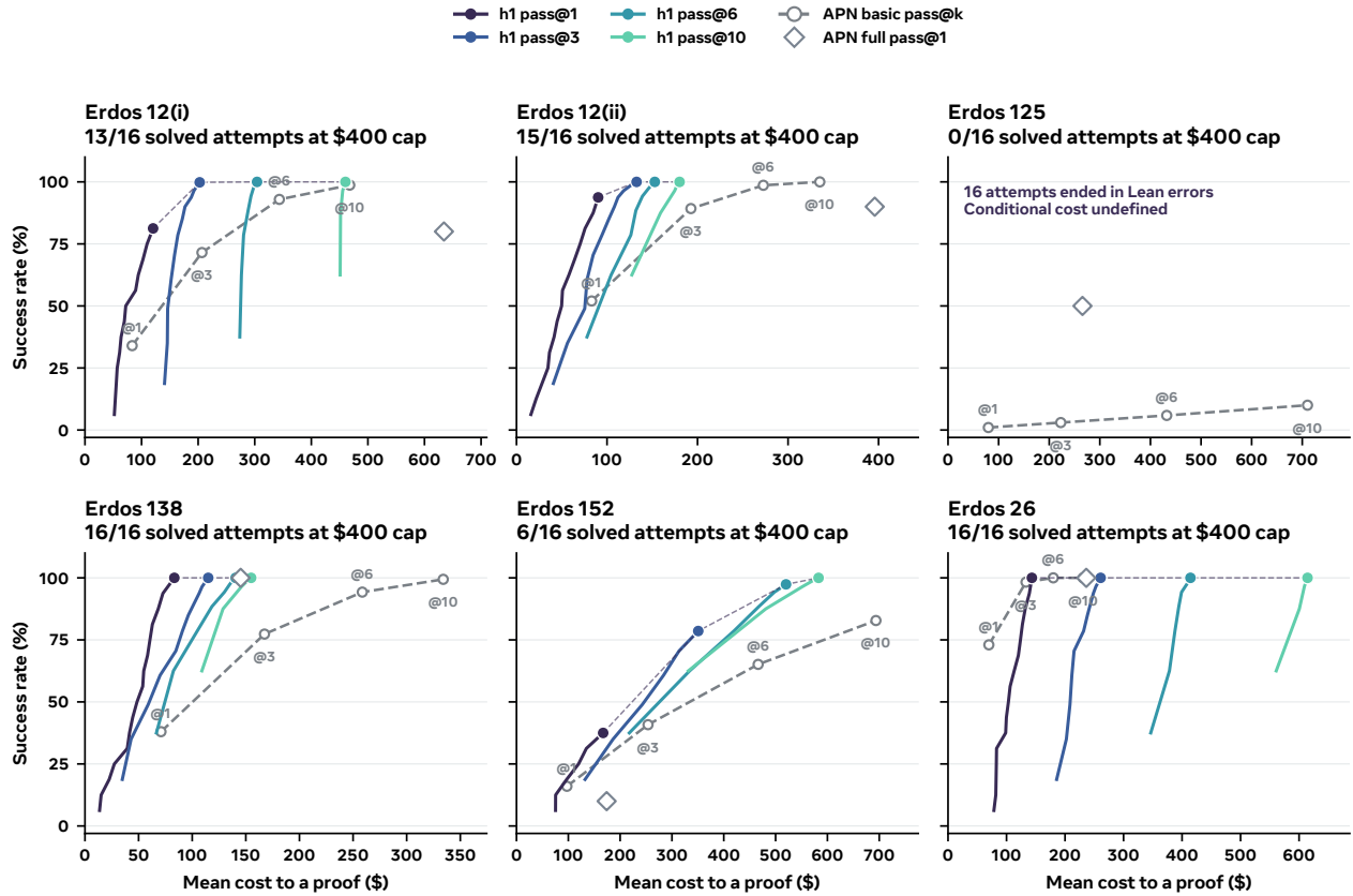
Figure 9 The five Erdős problems in Figure 1 (middle), plus Erdős 125. Solid coloured curves vary the active-time cutoff within an attempt, separately for each pass@ k ; filled circles mark terminal results. The dashed connection between those circles shows repetition at the final allowance. Grey circles are APN basic’s published pass@ k points, and the hollow diamond is APN full’s pass@1. All use Gemini 3.1 Pro. Horizontal scales differ across panels. Following AlphaProof Nexus (Tsoukalas et al., 2026), we report cost conditional on success. All 16 h1 replicas on Erdős 125 ended in Lean REPL timeout errors, so its conditional cost is undefined. Errors count as failures. APN full also uses AlphaProof, whose cost is absent from the published coordinates.
