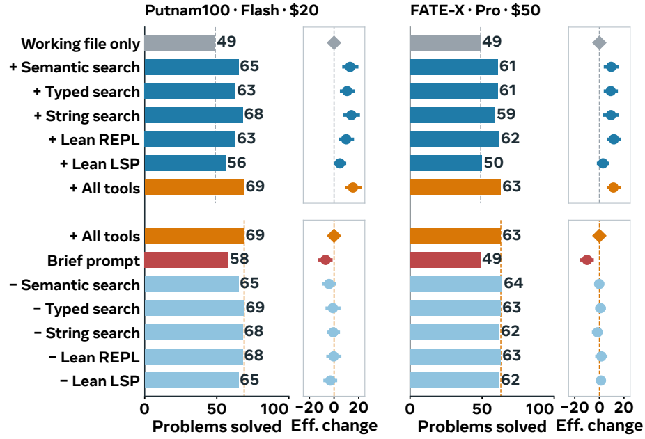
Figure 22 Tools provide overlapping benefits. Individual search tools or the REPL recover most of the full tool set’s gains; removing any single tool has little effect on coverage. Results cover the PutnamBench subset with Gemini 3 Flash and FATE-X with Gemini 3.1 Pro.
