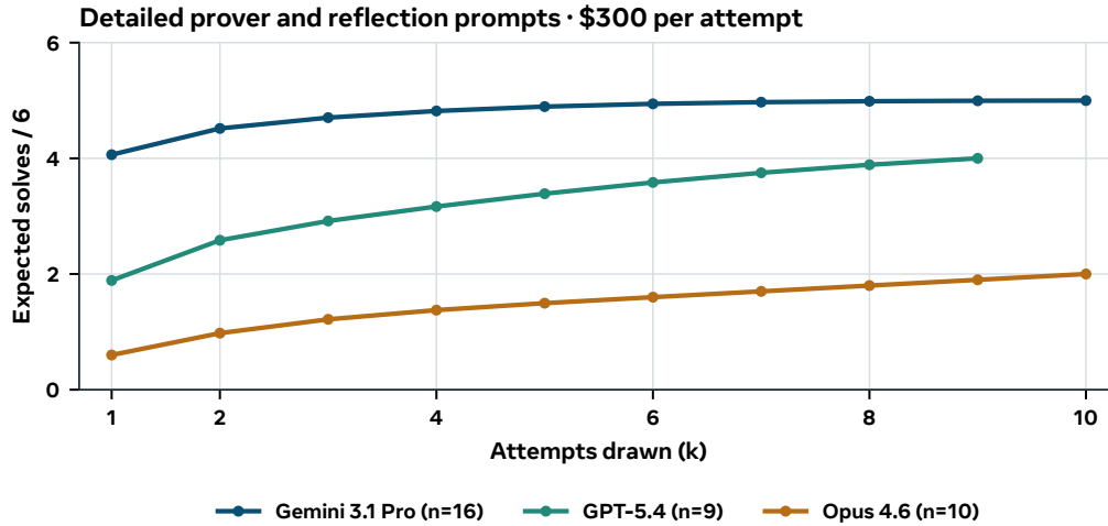
Figure 11 Model scaling on six Erdős problems with detailed instructions. All models use a $300 per-attempt cap. Curves sum per-problem pass@k estimates; Gemini 3.1 Pro has 16 replicas, GPT-5.4 nine, and Opus 4.6 ten.
