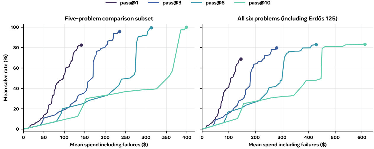
Figure 13 Longer h1 attempts can be cheaper than repetition even when failures are charged. All curves use Gemini 3.1 Pro in the same harness. Lines join nondominated observed points as the per-attempt dollar cap varies; circles mark terminal results. Cost averages successful and unsuccessful groups, with cancellation at the first accepted proof in successful groups. Left: the five-problem subset used in Figure 1. Right: all six problems, including Erdős 125 with zero accepted attempts and its recorded costs. Its unconditional mean cost remains defined even with no successful attempts, whereas its conditional cost is undefined. Solve rates and costs give each problem equal weight.
