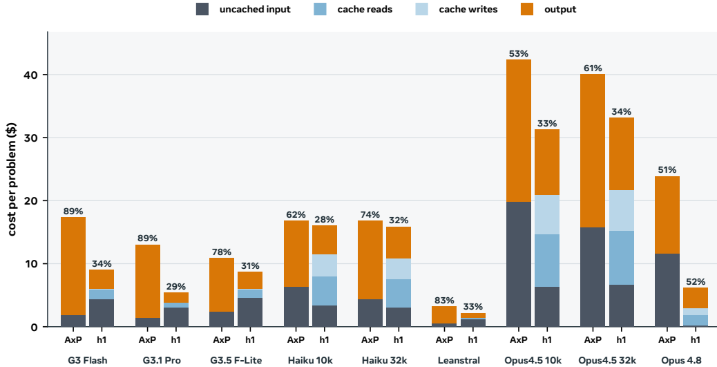
Figure 18 Cost per problem by token type, PutnamBench subset, nine model settings under AxProverBase (AxP) and h1. Bars average costs across solved and unsolved problems. Percentages show output tokens' share of total cost.
