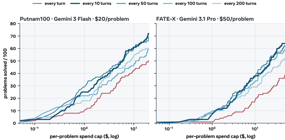
Figure 27 Solve rates at different budgets and reflection intervals. Reflection follows every 1, 10, 50, 100, or 200 proof-search turns ( T_1 – T_{200} ). Gemini 3 Flash is evaluated on the PutnamBench subset at up to $20 per problem (left), and Gemini 3.1 Pro on FATE-X at up to $50 (right). Reflection every turn produces fewer solves over most observed budgets; intervals of 10 and 50 turns give similar curves.
